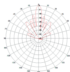
Horizontal Polarization
