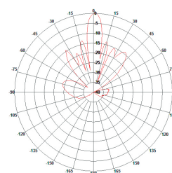
Horizontal Polarization
