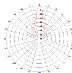
E-Plane Pattern
